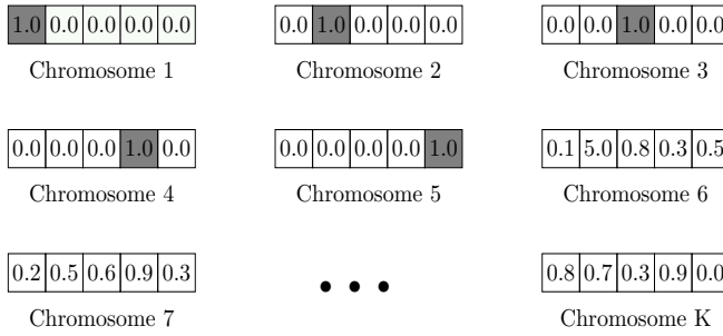
Fig. 4: Illustration of GA population initialisation for N_\theta = 5 thresholds.
