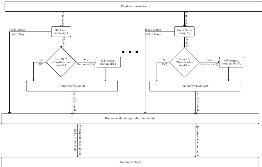
Fig. 3: Our proposed multi-threshold strategy framework. It uses a majority vote system to sum similar trade action recommendations from thresholds and it follows the action with the highest sum. The action is taken after calculating the weighted average of the forecasted trend reversal point of thresholds that recommended the winning action.
