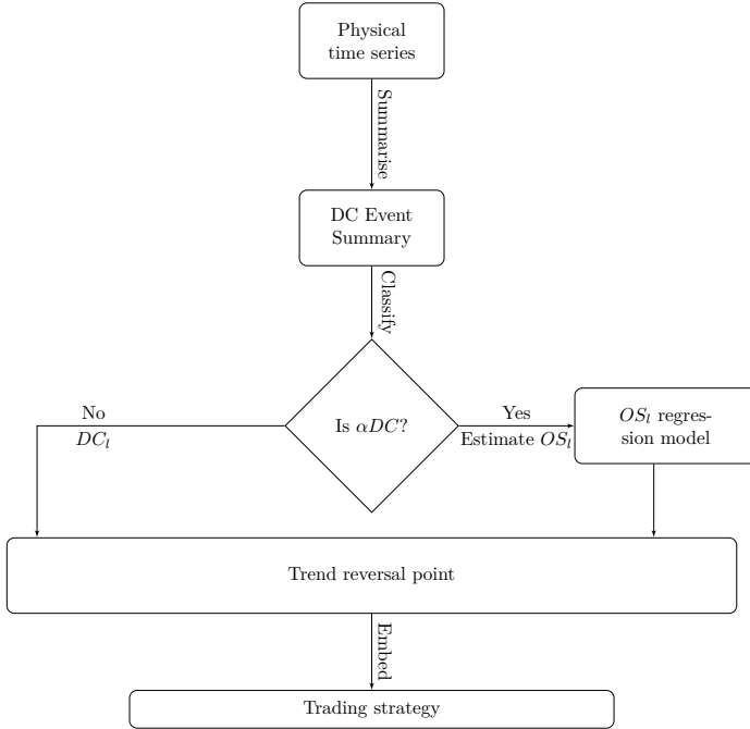
Fig. 2: Predicting trend reversal in DC. A DC trend classified to compose of only DC event is expected to reverse at DCC, while DC trend classified to compose of DC and OS events is expected to reverse at estimated DCE, which is the sum of DC event length at DCC and the OS event length predicted by the SRGP. Once the trend reversal point has been determined, we embed it into a trading strategy and perform trading.
