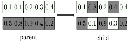
Fig. 5: A sample uniform crossover operation by our GA. Either of the children is randomly selected for the next generation
