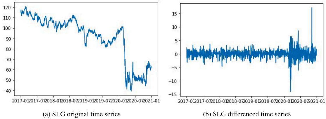
Fig. 1. Differencing example.
